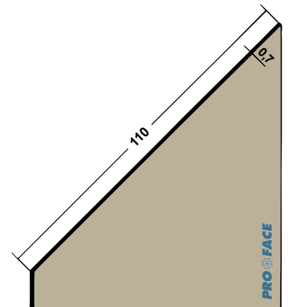
Proface®-YOIN-FLEX FL1100S-P
