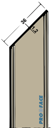
Proface®-YOIN-FLEX FL360-P
