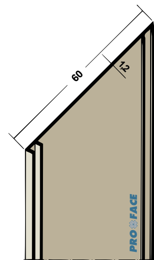
Proface®-YOIN-FLEX FL600M-P
