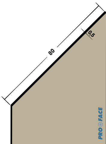
Proface®-YOIN-FLEX FL800S-P
