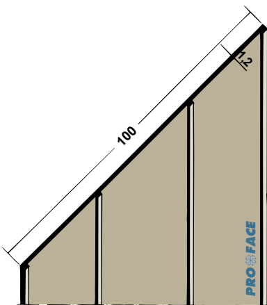
Proface®-YOIN-FLEX FL1000-P
