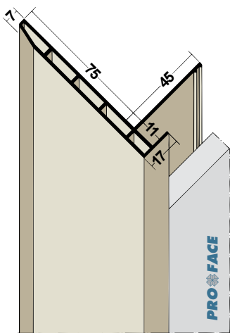
Proface®-YOIN-U U860SH-P
