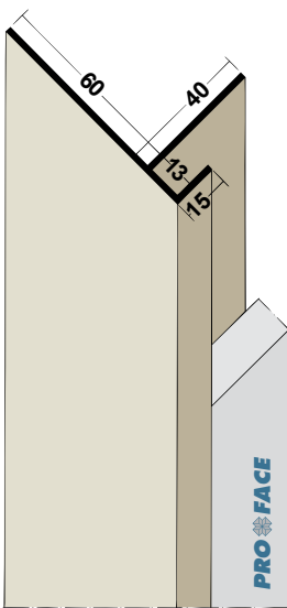
Proface®-YOIN-U U730S-P
