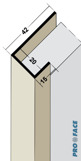
Proface®-YOIN-U U200-P
