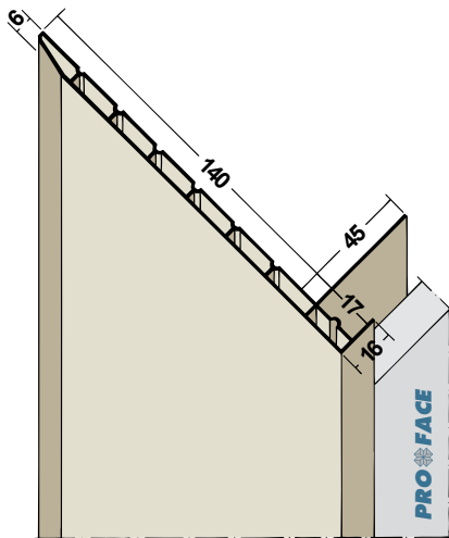
Proface®-YOIN-U U1570SH-P
