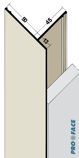
Proface®-YOIN-U U630S-P
