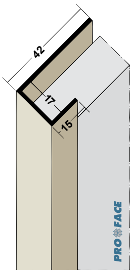
Proface®-YOIN-U U170-P
